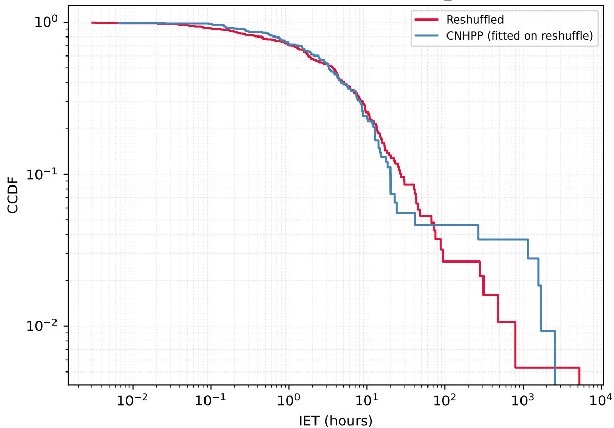
User 2047003776 - Reshuffled vs CNHPP A_{\text{fit}}=1.1021
